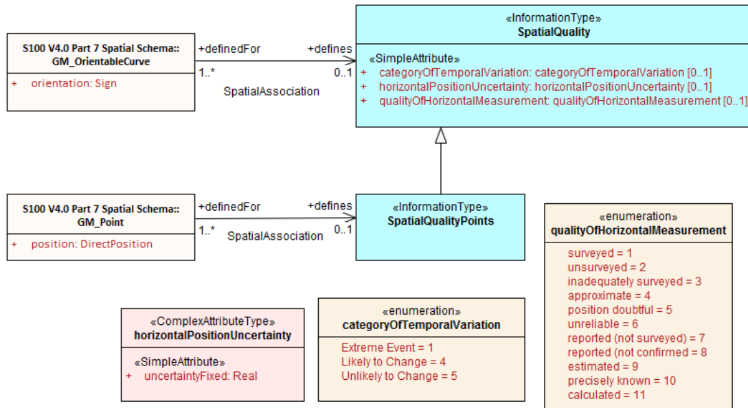
Figure 26. Spatial quality
