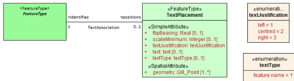
Figure 27. Text placement
