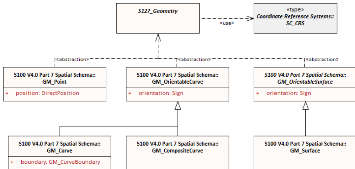
Figure 29. Geometric primitives
