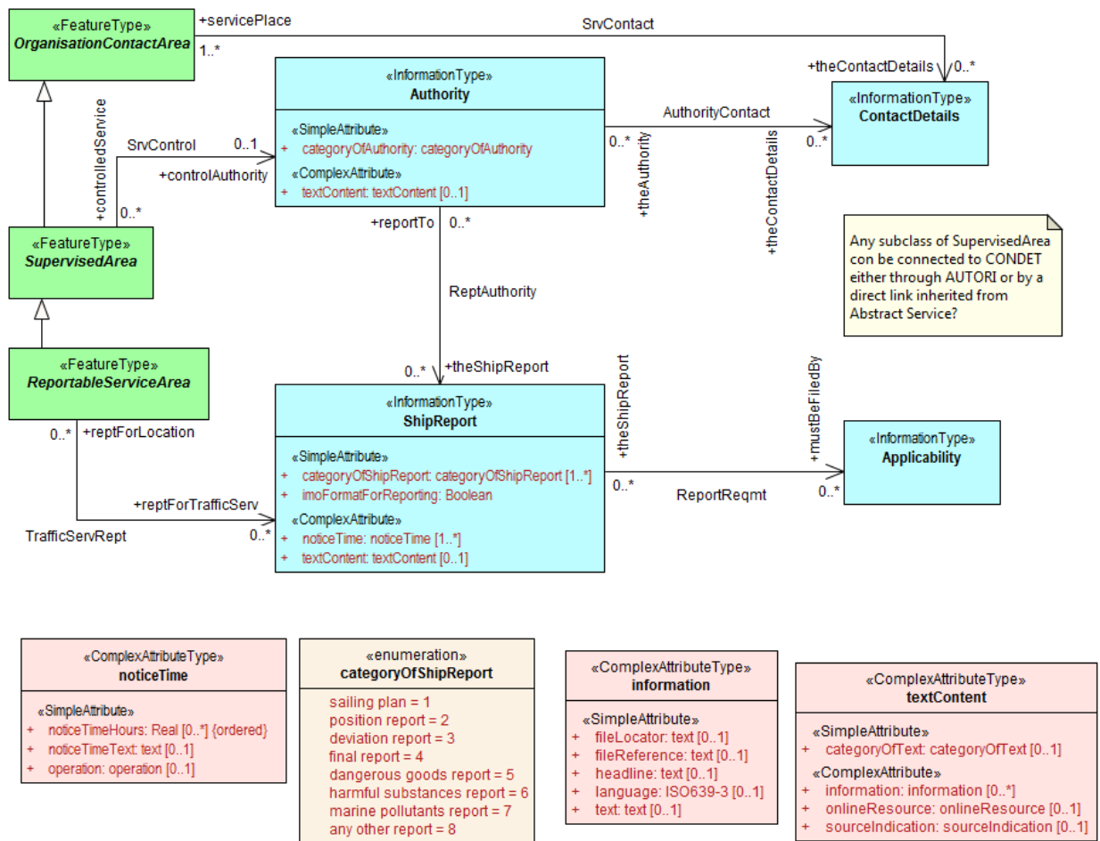
Figure 11. Reporting
