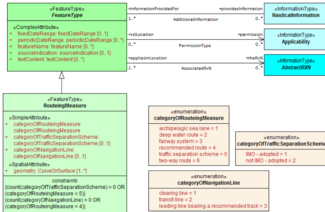
Figure 15. Routeing measures
