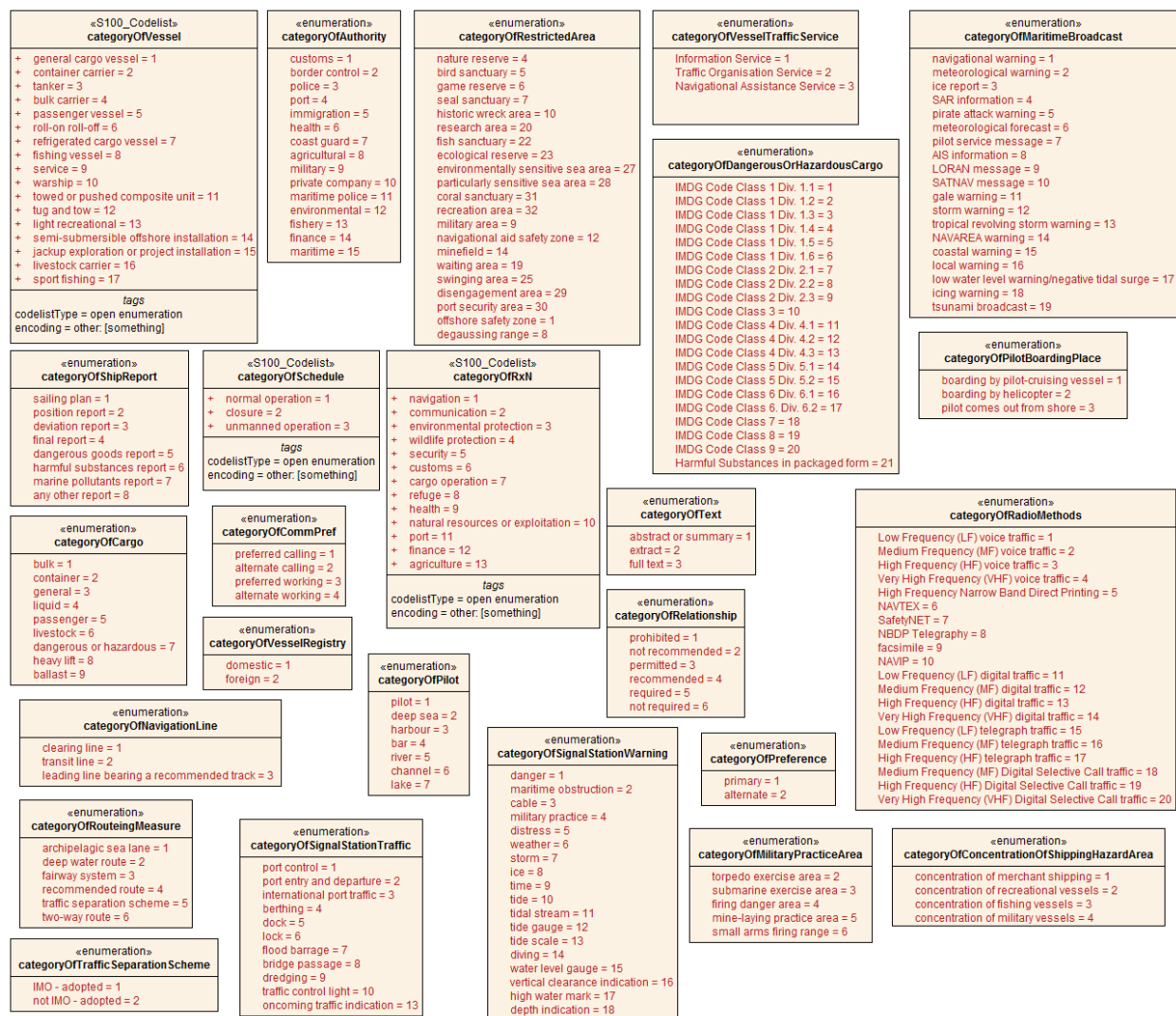
Figure 21. Category enumerations
