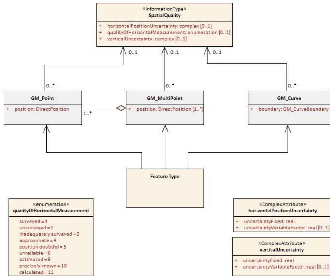
Figure 5 - Spatial Quality Information Type
