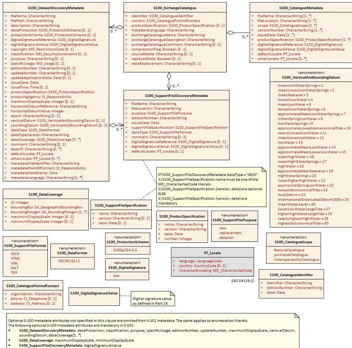
Figure 26 S-101 Exchange Set - Class Details
