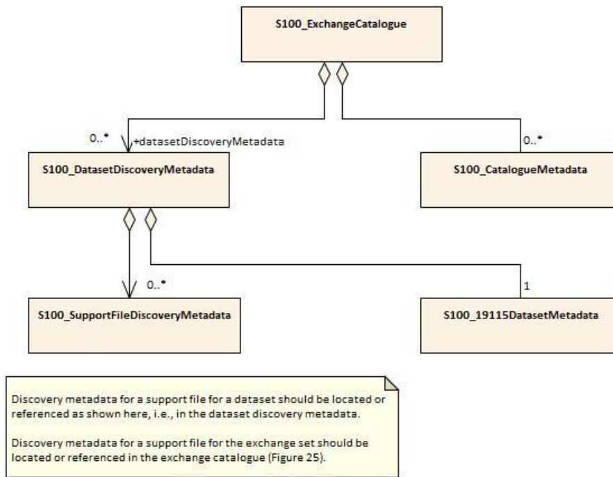
Figure 24 – S-101 Exchange Set Catalogue
