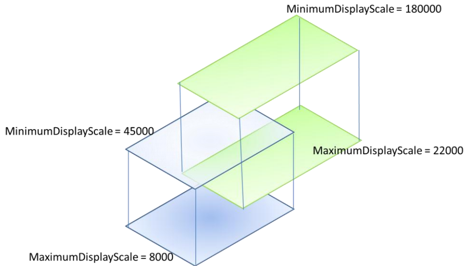
Figure 7 - Data Coverage Rules
