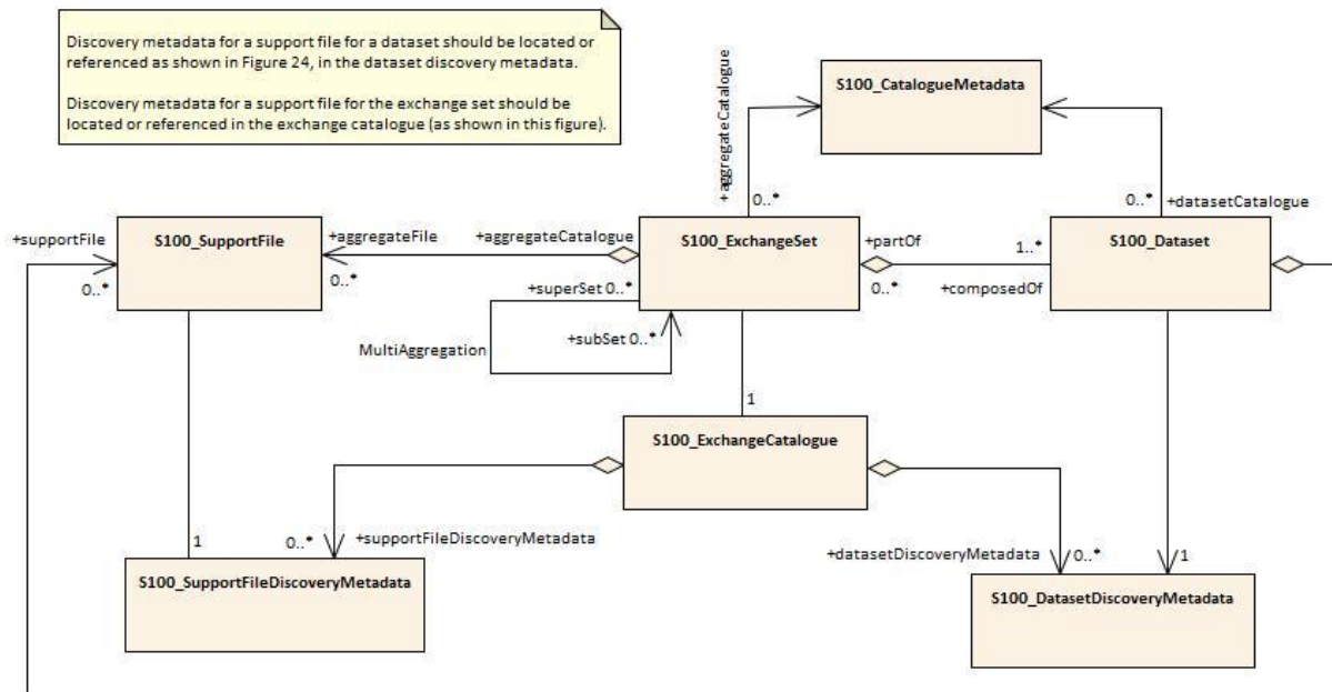
Figure 25 - S-101 Exchange Set
