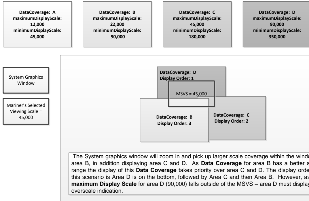
Figure 11 - Scenario 3: Display of three different overlapping Data Coverages
