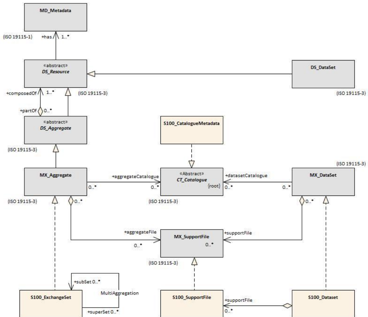
Figure 23 Realization of the Exchange Set Classes
